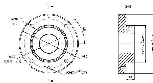
LA906-7H Hollow Wrist Type
