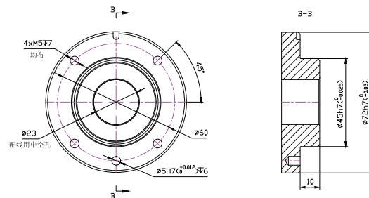
LA707-7H Hollow wrist type
